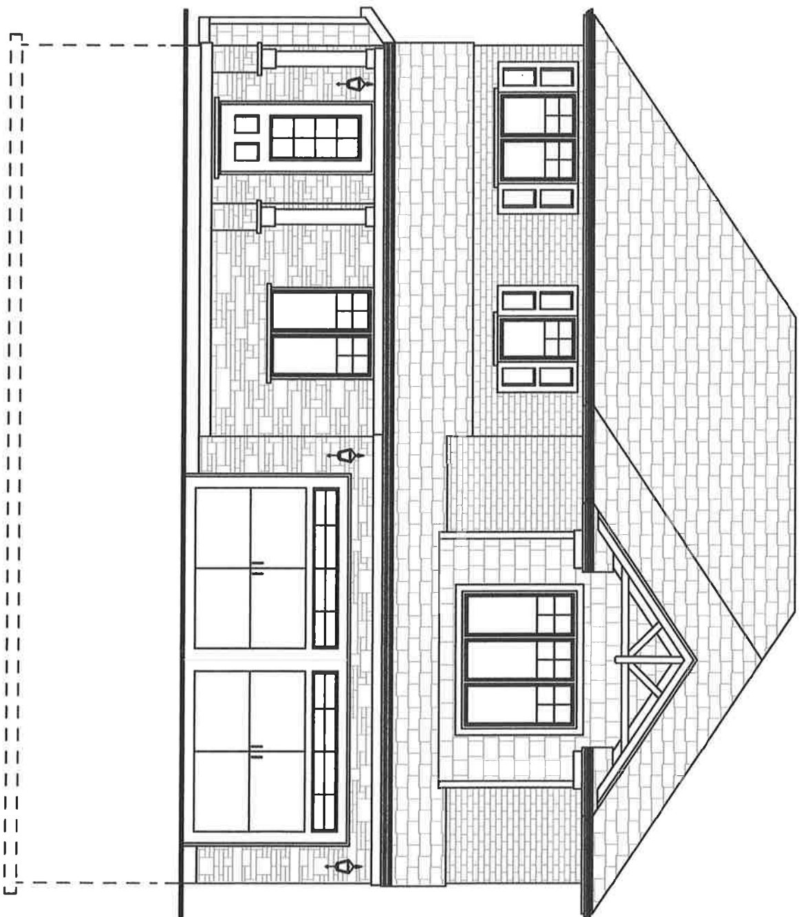
FRONT ELEVATION
